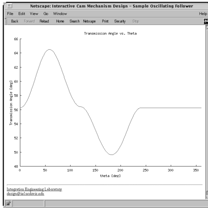
Figure 6.31: Transmission angle of the cam.
