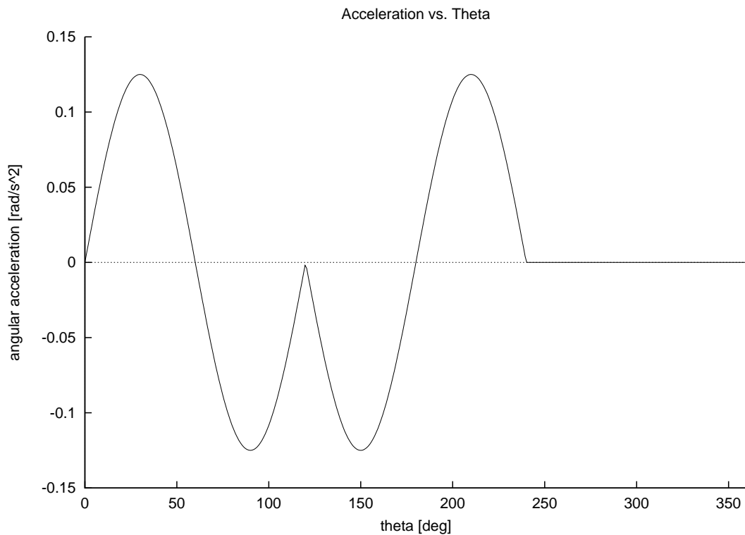
Figure 6.18: Oscillating follower acceleration.
