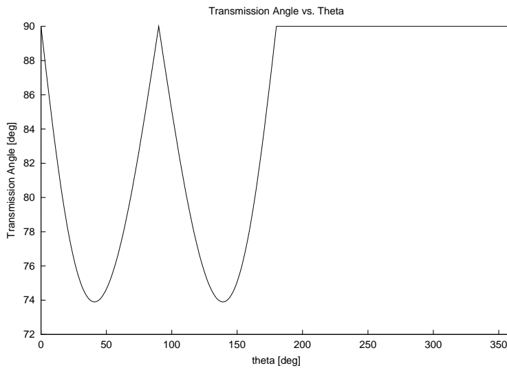
Figure 6.11: Transmission angle of the cam.
