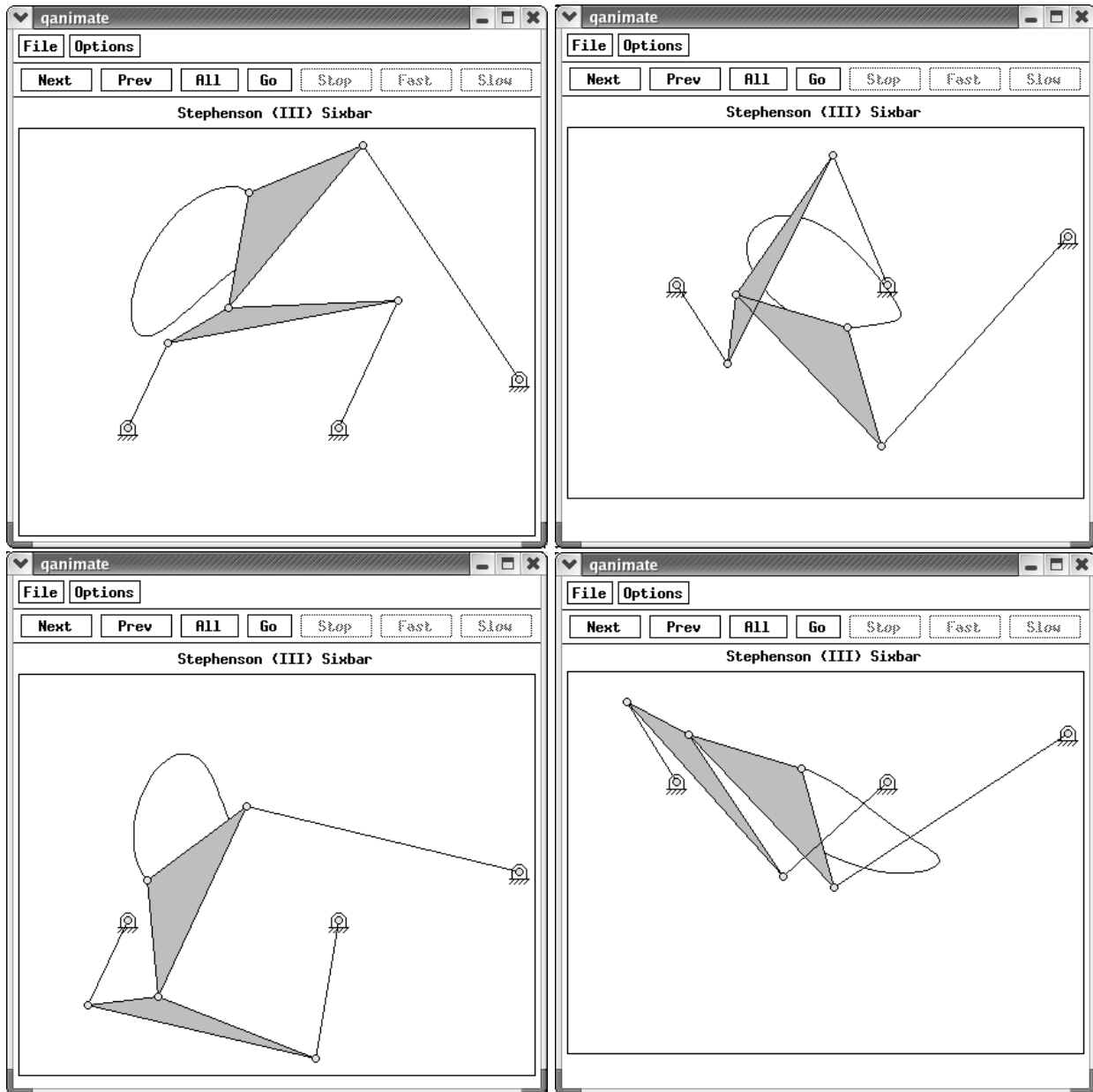
Figure 5.29: Output of Program 42.
