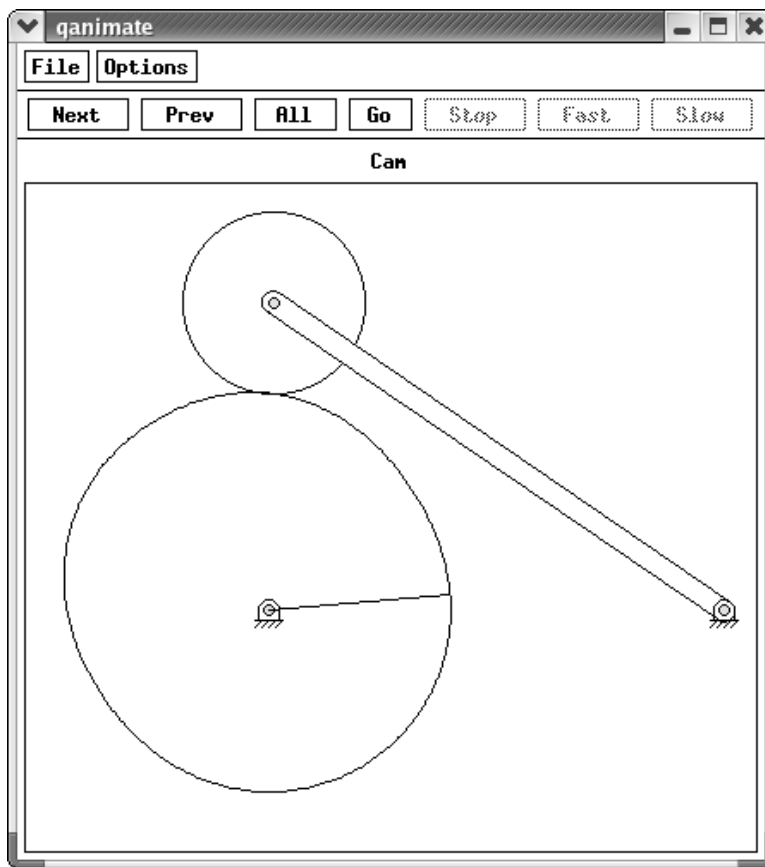
Figure 6.22: Animation of cam with Oscillating follower.
