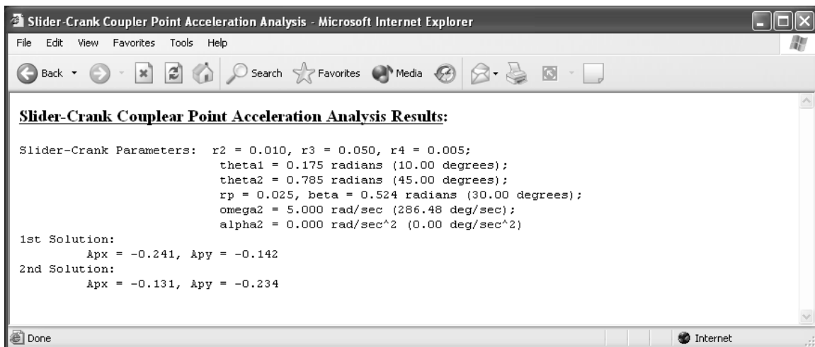
Figure 3.23: Output of coupler point acceleration analysis.
