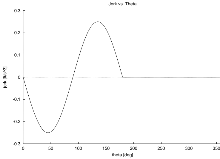
Figure 6.10: Translating follower jerk.
