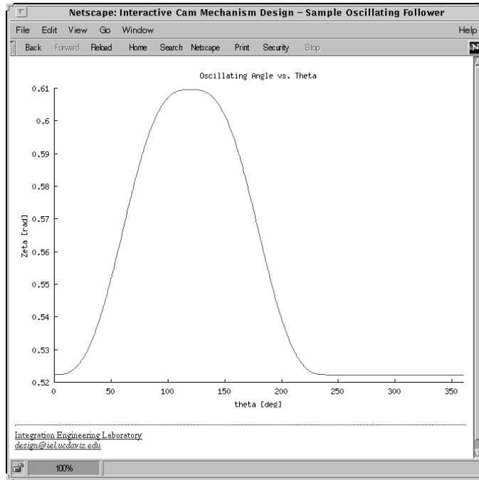
Figure 6.28: Oscillating follower position.
