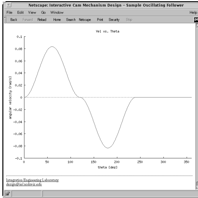
Figure 6.29: Oscillating follower velocity.
