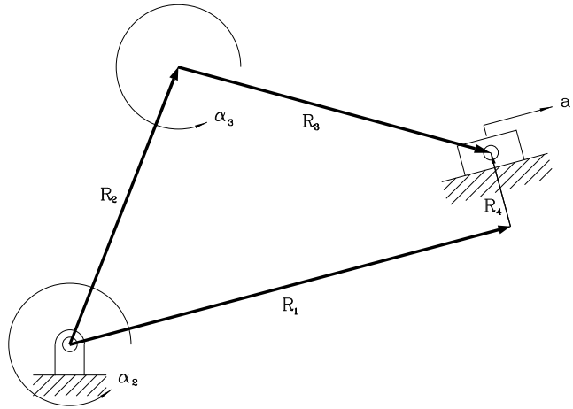
Figure 3.7: Accelerations for a crank-slider mechanism.
