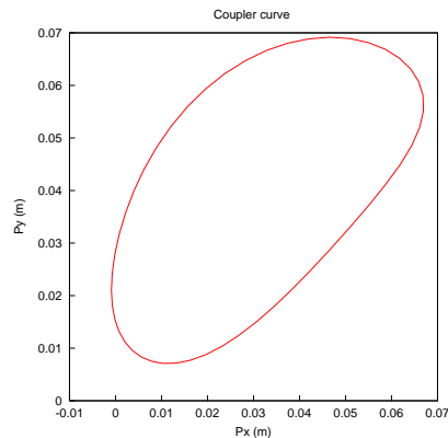
Figure 1.2: A coupler curve for a crank-rocker four-bar linkage.
