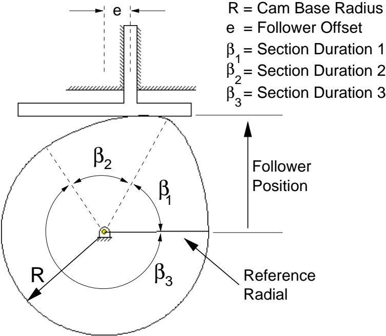
Figure 6.1: Translating flat-faced follower parameters
