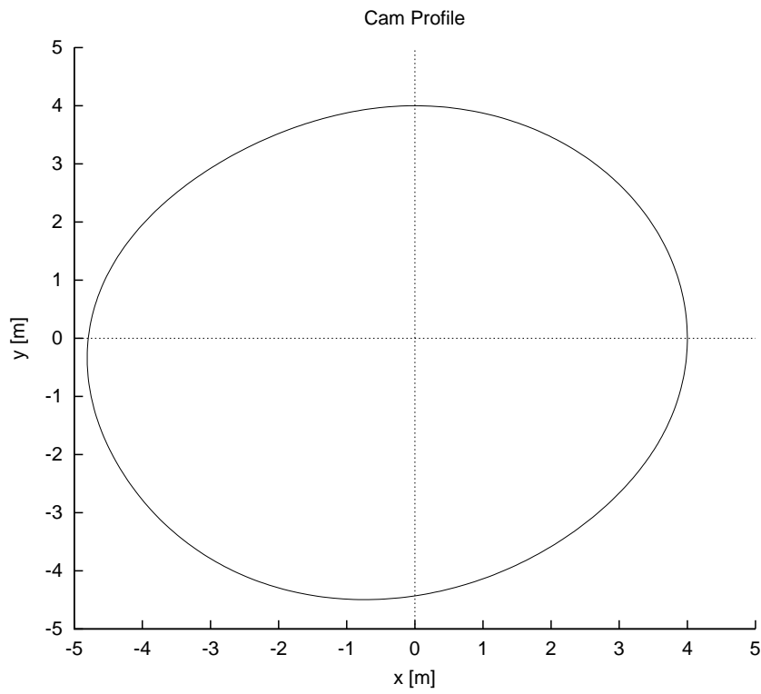
Figure 6.21: Cam profile.
