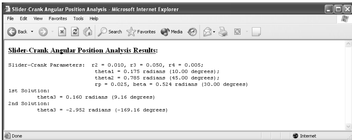
Figure 3.15: Output of angular position analysis.
