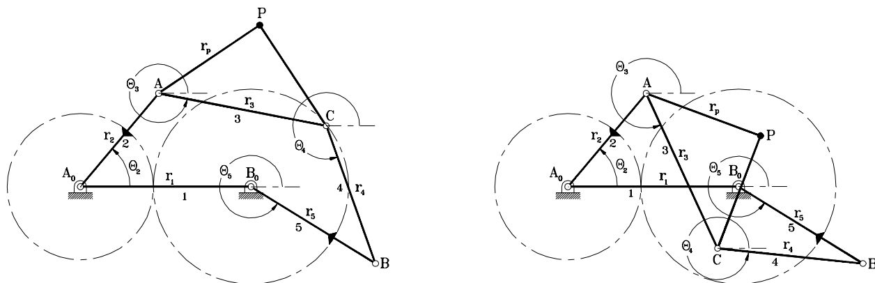
Figure 4.1: Both Inversions of the Geared Fivebar Linkage
