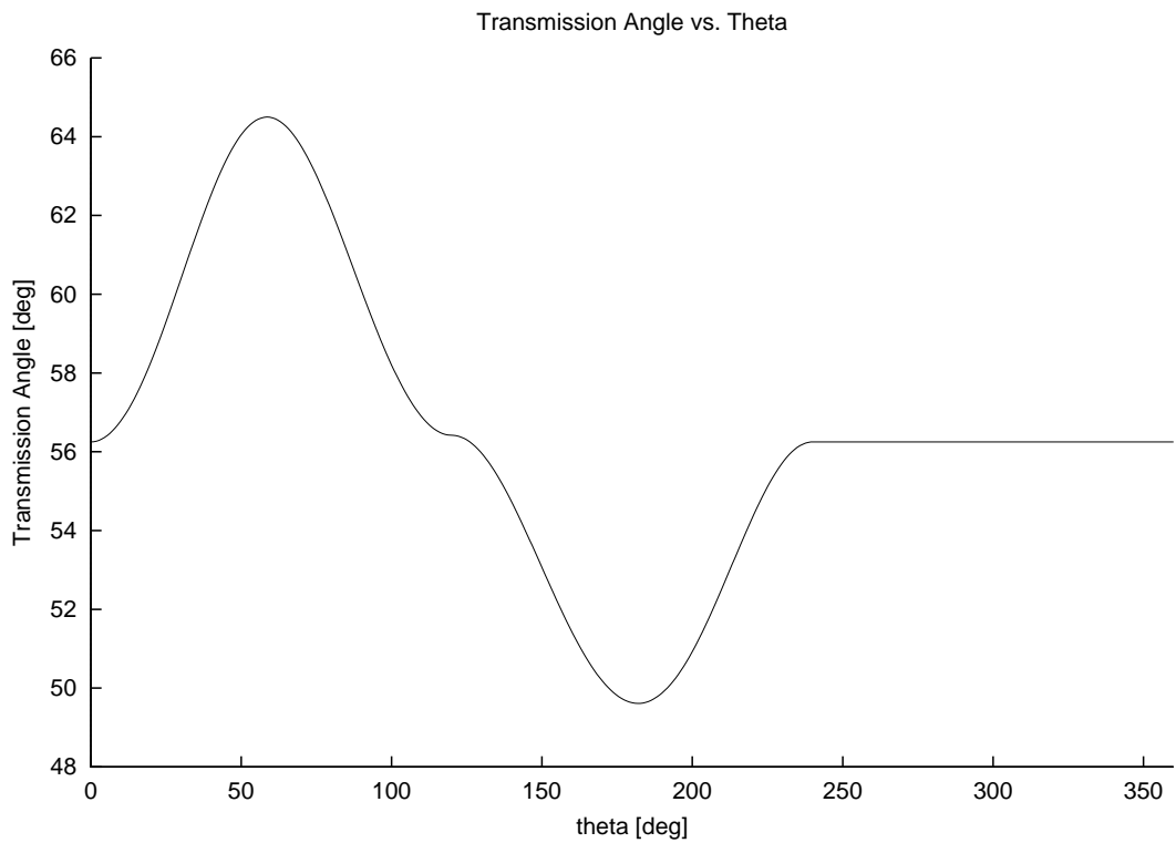
Figure 6.20: Transmission angle of the cam.
