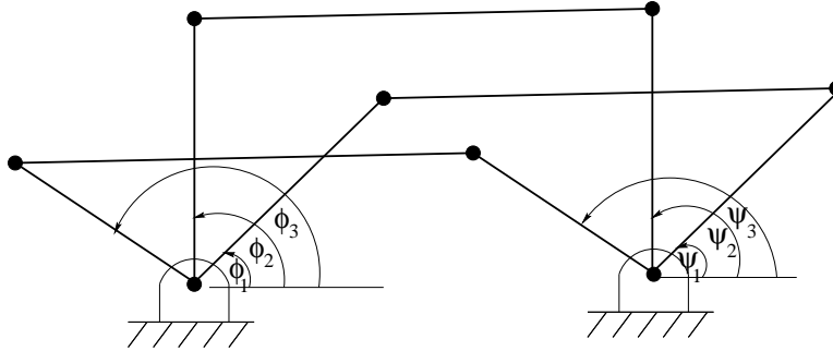
Figure 2.12: Freudenstein analysis.
