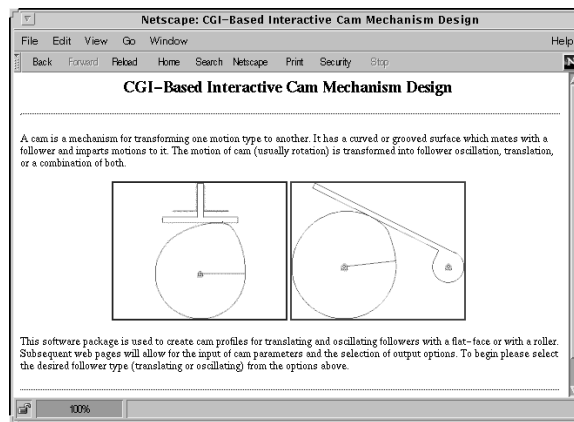
Figure 6.23: Opening cam synthesis page
