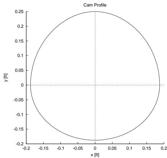
Figure 6.12: Cam profile.
