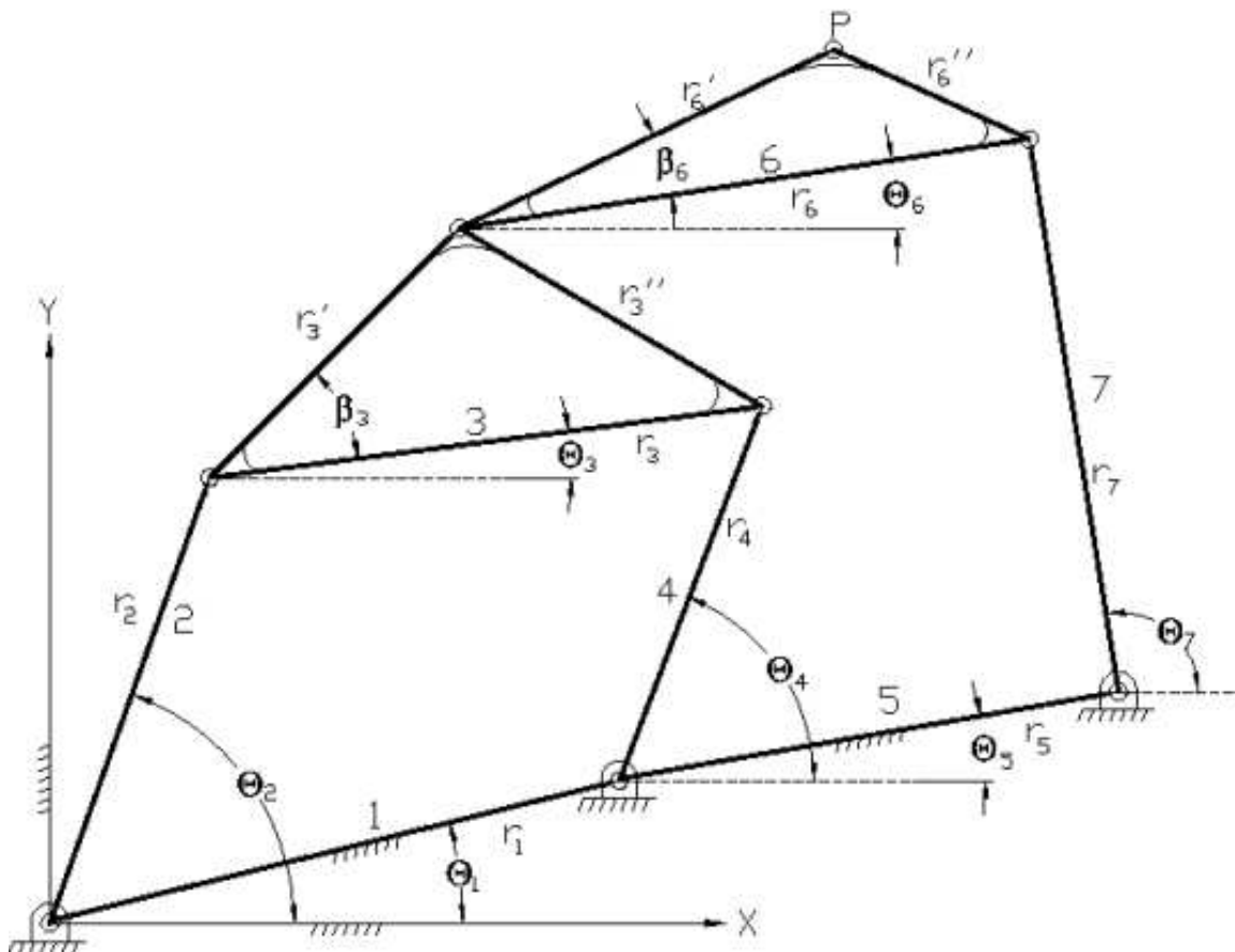
159 Figure 5.28: Stephenson (III) Sixbar Linkage
