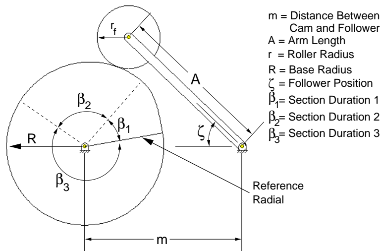
Figure 6.4: Oscillating roller follower parameters
