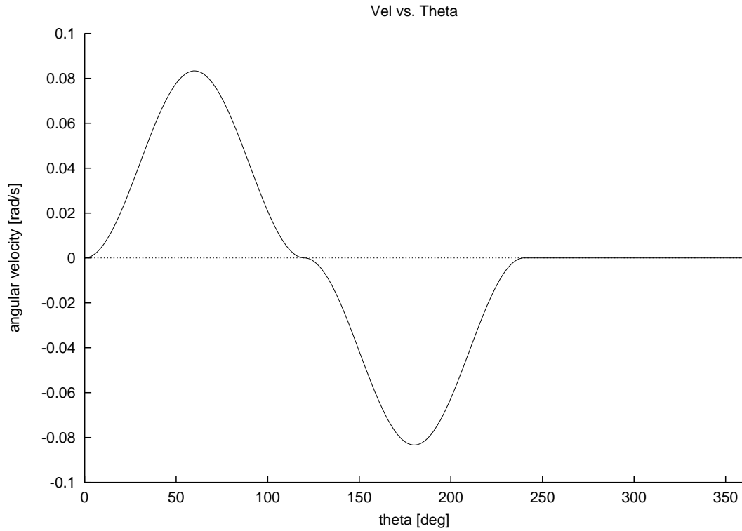
Figure 6.17: Oscillating follower velocity.
