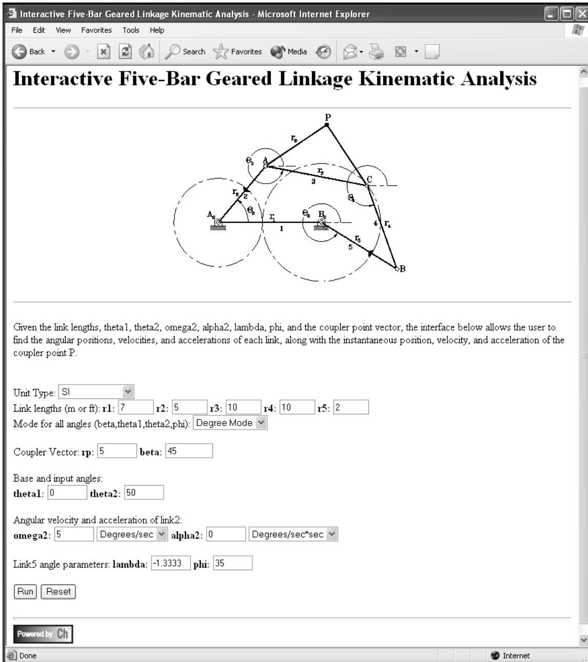
Figure 4.4: Web-based geared fivebar linkage analysis.
