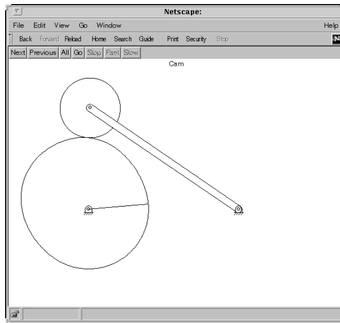
Figure 6.33: Animation of cam with Oscillating follower.
