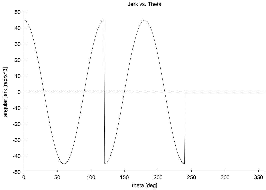
Figure 6.19: Oscillating follower jerk.
