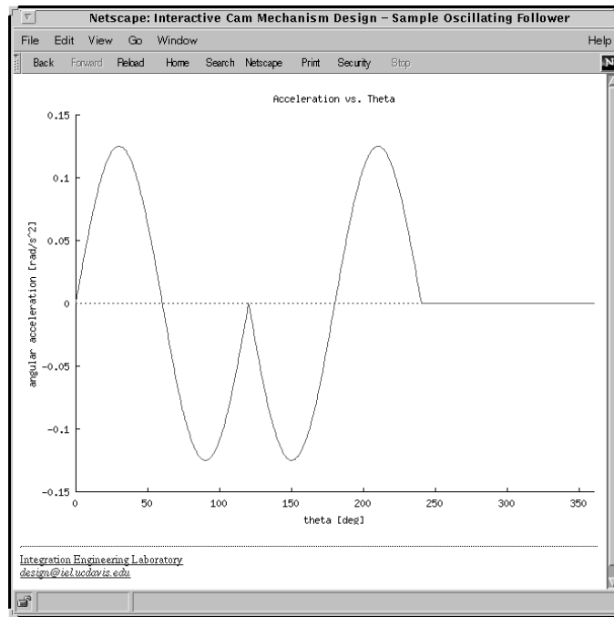
Figure 6.30: Oscillating follower acceleration.
