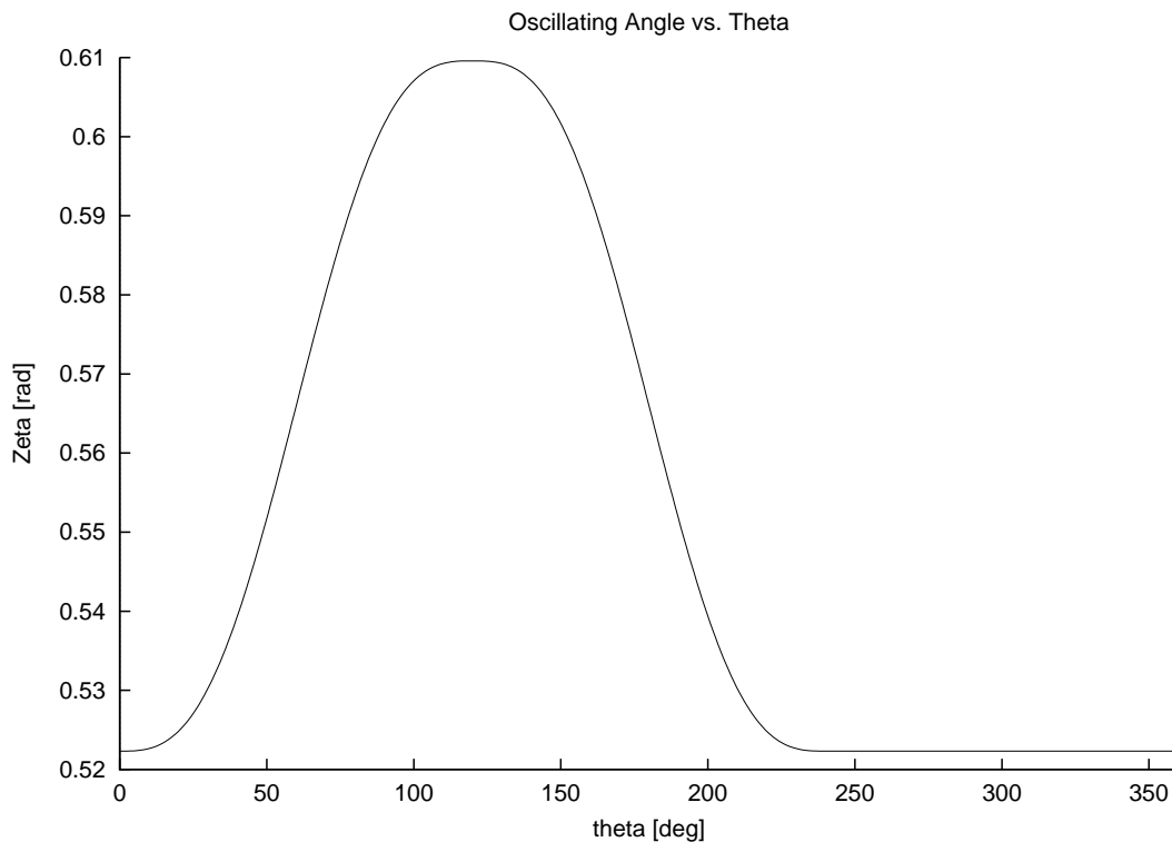
Figure 6.16: Oscillating follower position.
