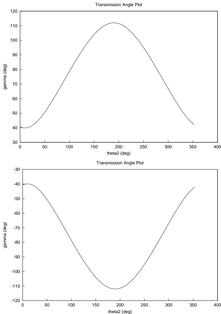
Figure 2.5: Transmission angle plots.
