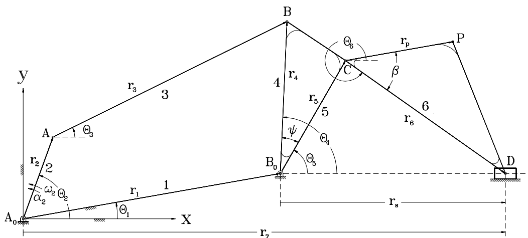
Figure 5.1: Barslider Linkage
