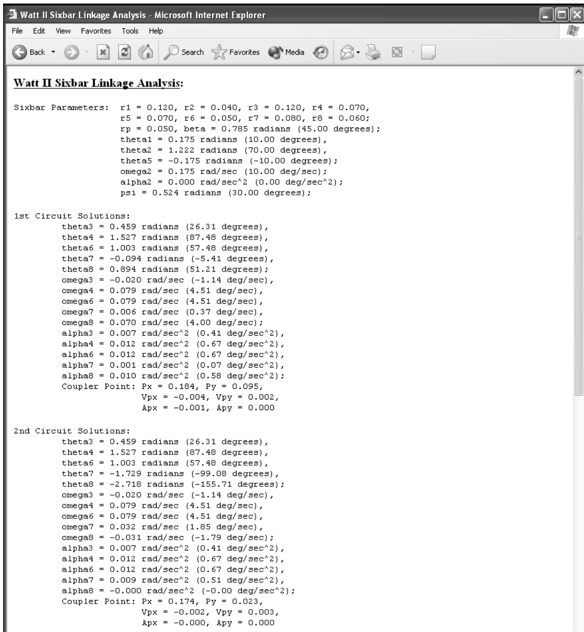
Figure 5.19: Output of web-based Watt (II) sixbar kinematic analysis.
